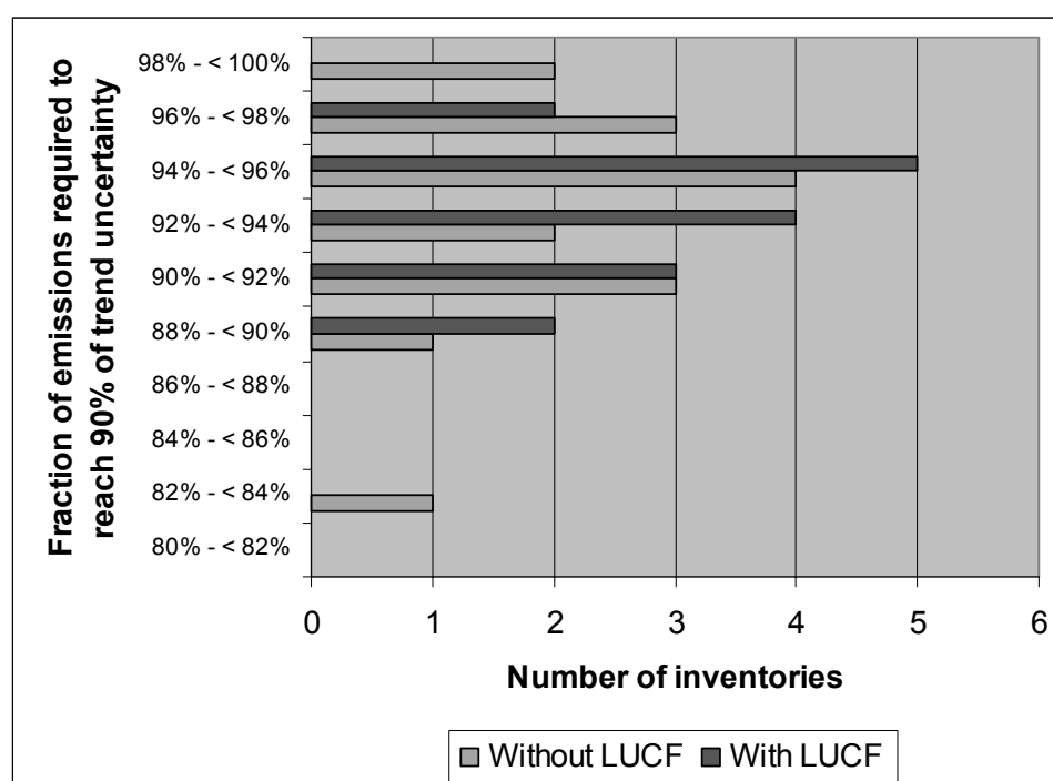
Figure 5.4.5 Fraction of emissions required to reach 90 % of sum of contribution from trend uncertainty in different inventories. With and without LULUCF (with LULUCF using absolute values of emissions).
