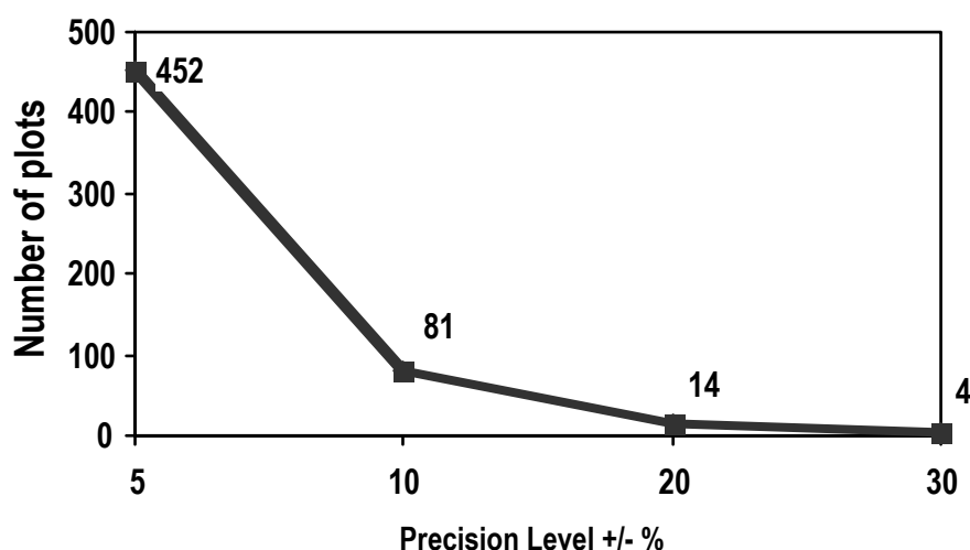
Figure 4.3.1 An example of the relationship between the number of plots and the precision level (+/- % of total carbon stock in living and dead biomass, with 95% confidence) for all strata combined, for a complex tropical forest in bolivia (the Noel Kempff Pilot Project); the project encompassed six strata and 625 plots were actually installed (from data in Boscolo et al., 2000 and Brown et al., 2000a).
