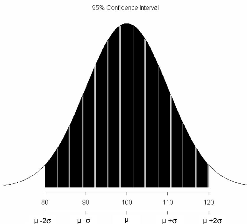
Box 5.2.1 EXAMPLE OF UNCERTAINTY EXPRESSION
