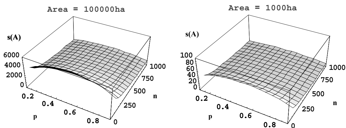
Figure 5.3.4 Relationship between the standard error of the area estimate s(A) , the proportion of the land-use class p , and the sample size n
