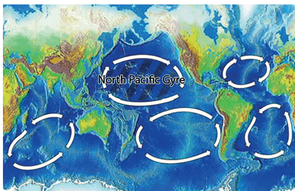
Figure 15 The area of increased plastic particles is located within the North Pacific Gyre, one of the five major ocean gyres. Credit: Fangz, https://upload.wikimedia.org/wikipedia/commons/6/64/North_Pacific_Gyre_World_Map.png .
