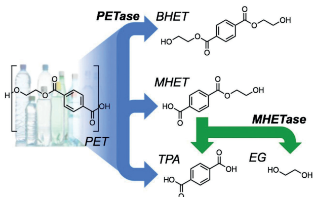
Figure 17 PETase catalyses the depolymerization of PET to bis(2-hydroxyethyl) - TPA (BHET), MHET, and TPA. MHETase converts MHET to TPA and EG. Reproduced with permission from Proceedings of the National Academy of Sciences (PNAS) (see ref. 201).
